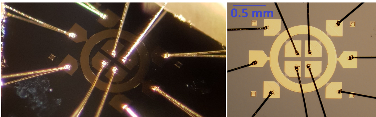
Figure 1: A photo taken under an angle (left) and a microscope image (right) of the multi-terminal Corbino device [4].
